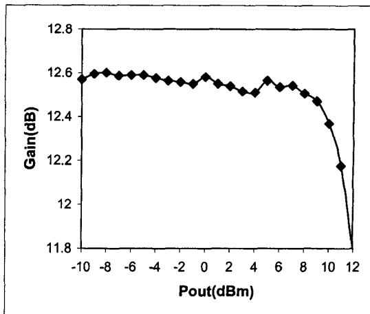
Figure 6. Power gain versus output power.
