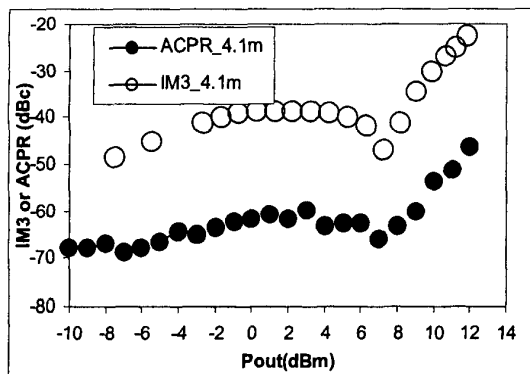
Figure 5. IM3 and ACPR versus output power.
