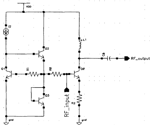
Figure 4. Simplified schematic of a PA driver circuit
